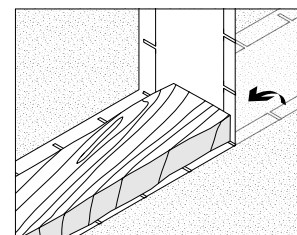
STEP 2 - Bend in the corner by hand and finish shaping with a rubber mallet. Placing a block of wood close to the fold improves the result.
